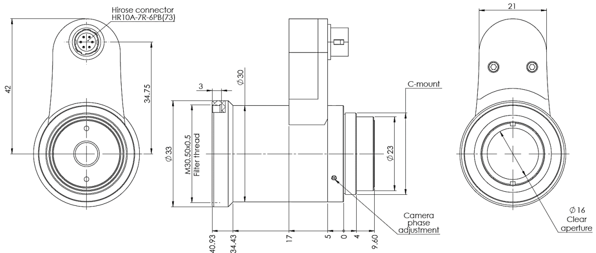
Figure 1: Mechanical drawing of the ELM-6-5.6-9-C
