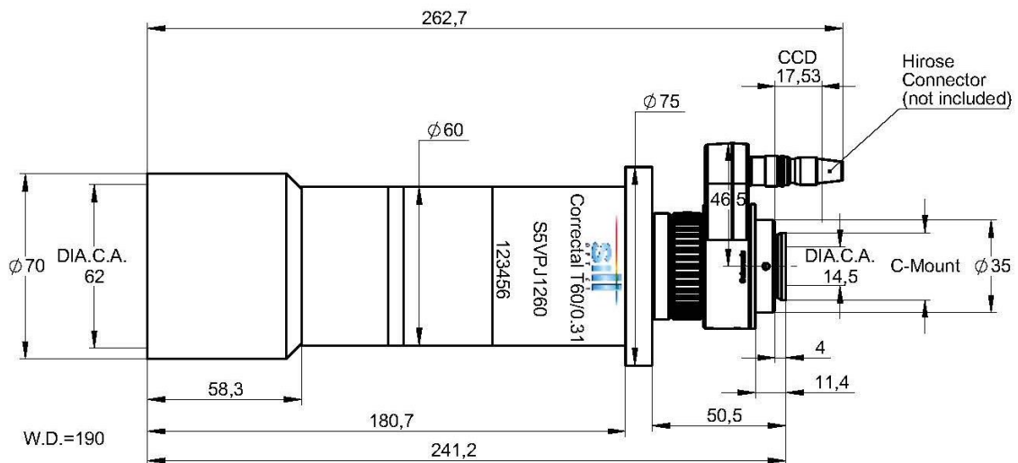
Figure 1: Mechanical drawing of the S5VPJ1260
