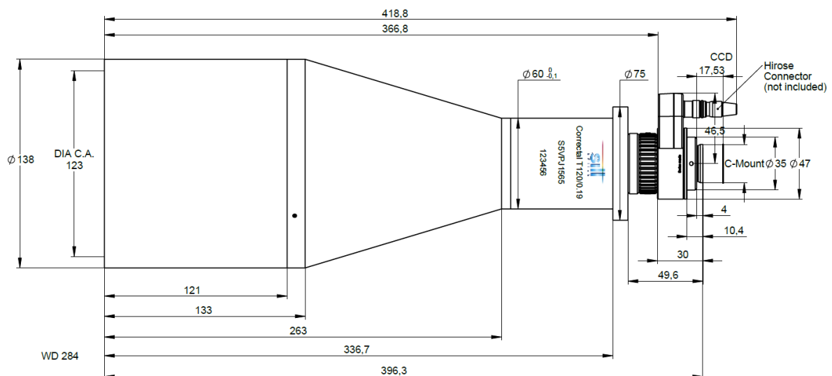
Figure 1: Mechanical drawing of the S5VPJ1565
