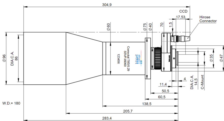
Figure 1: Mechanical drawing of the S5VPJ6060
