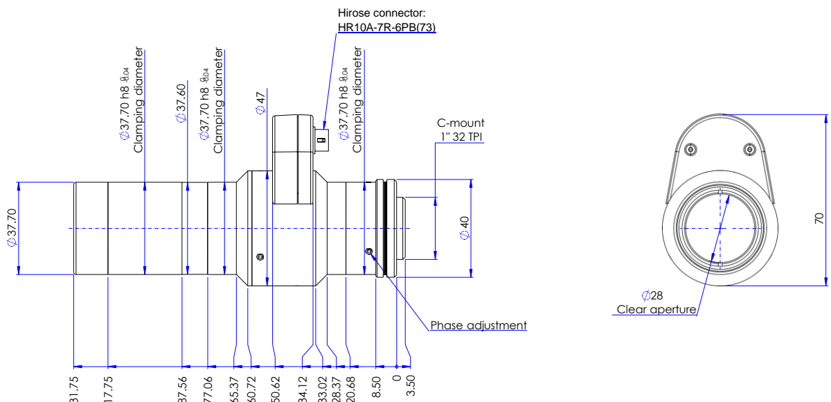
Figure 1: Mechanical drawing of the TCEL050
