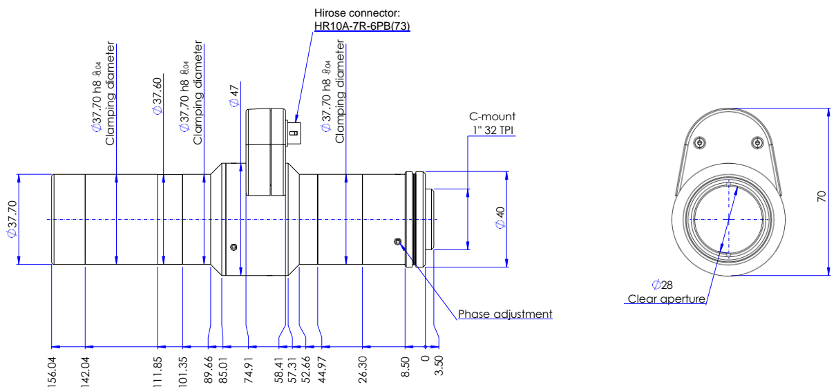
Figure 1: Mechanical drawing of the TCEL075
