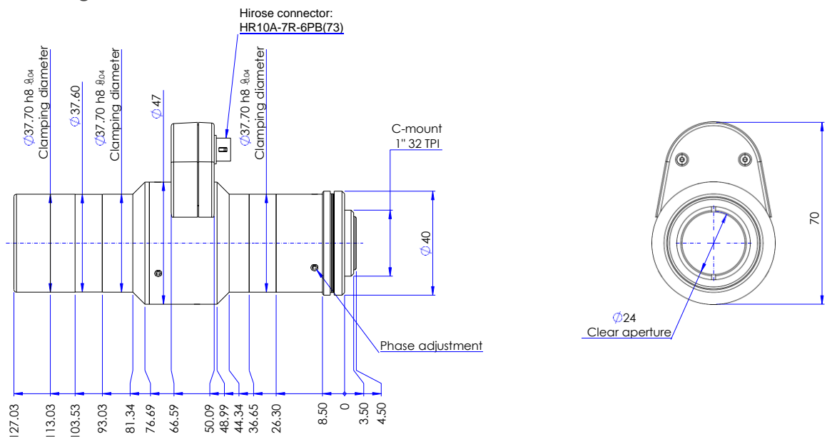
Figure 1: Mechanical drawing of the TCEL100
