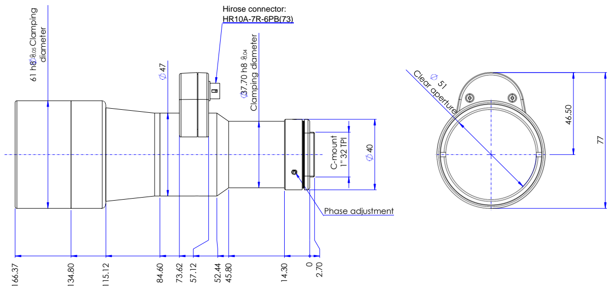
Figure 1: Mechanical drawing of the TCEL23036
