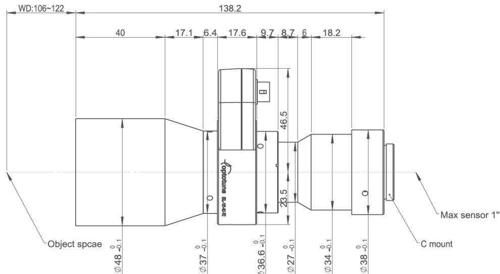
Figure 1: Mechanical drawing of the TS1-05-110-EL
