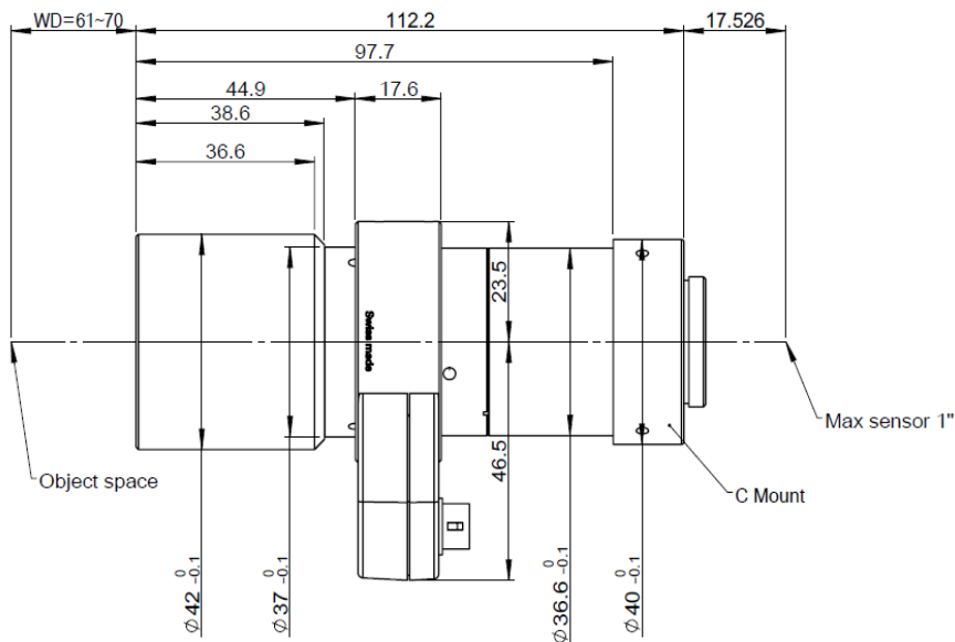
Figure 1: Mechanical drawing of the TS1-0638-70-EL
