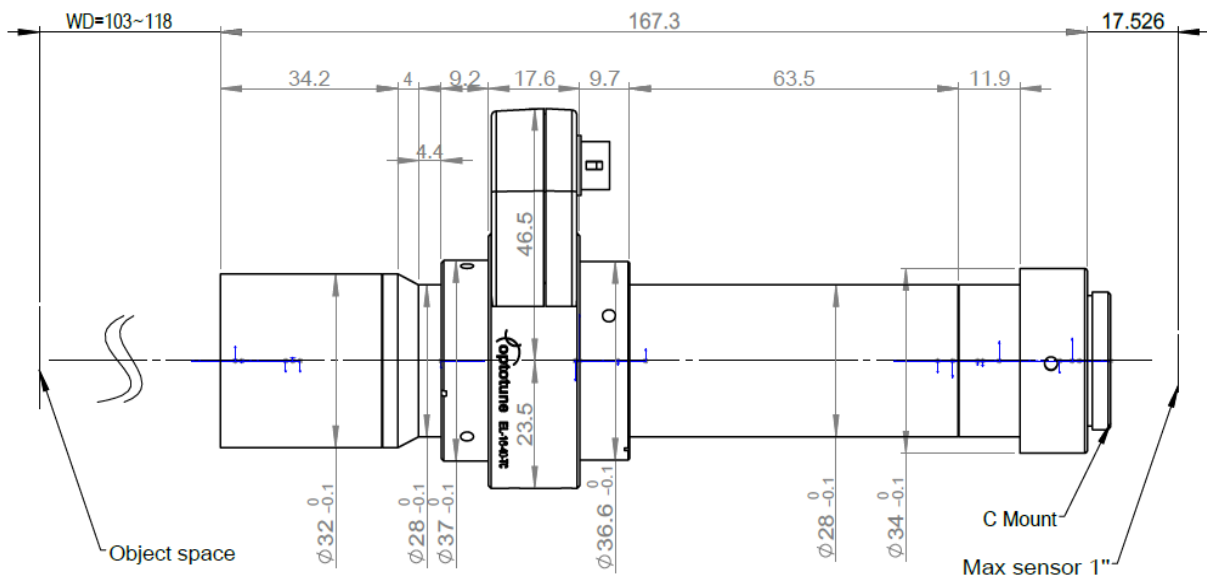
Figure 1: Mechanical drawing of the TS1-3.0-110-EL
