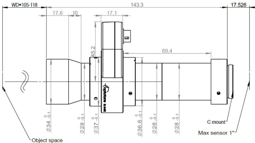
Figure 1: Mechanical drawing of the TS1-4.0-110-EL
