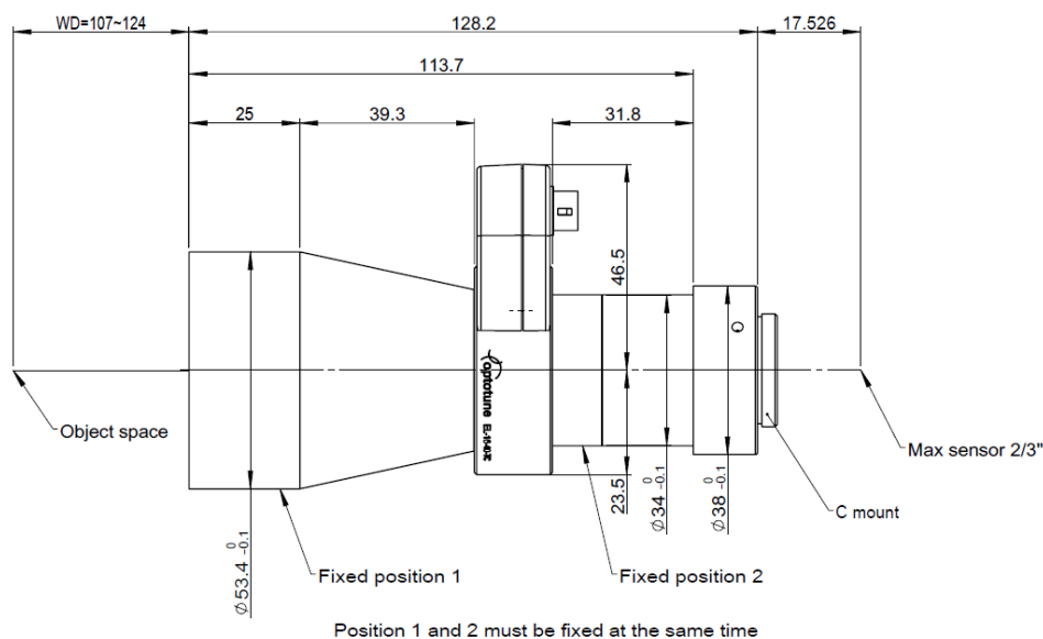
Figure 1: Mechanical drawing of the TS23-036-115-EL
