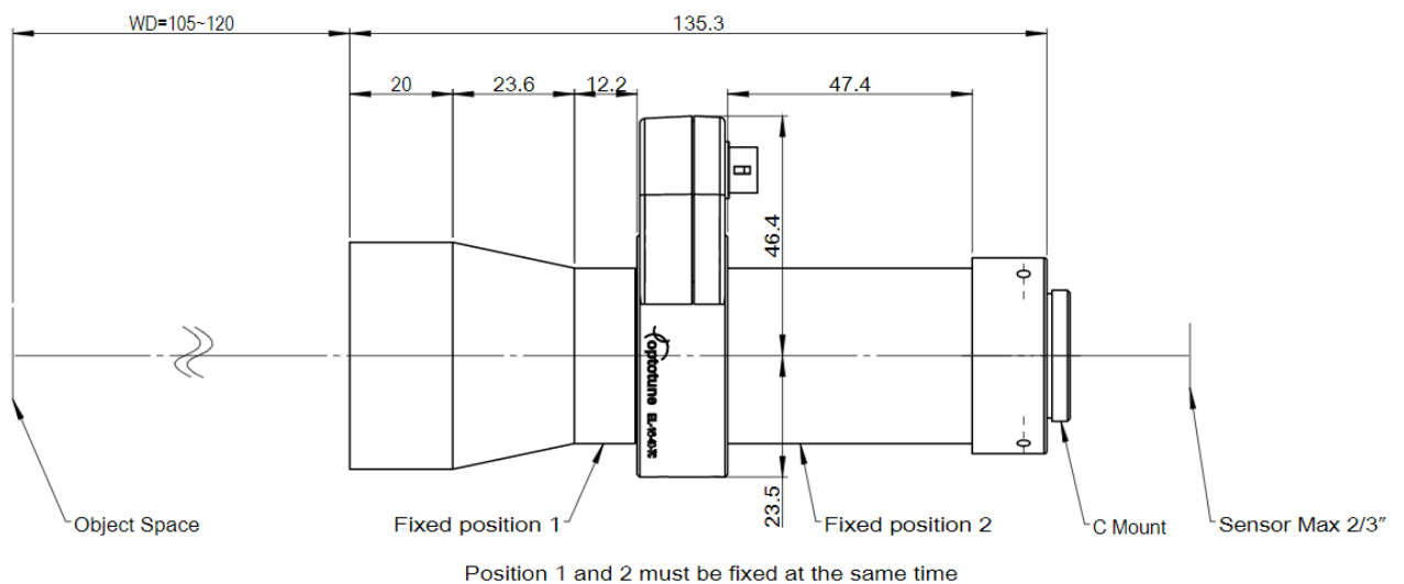
Figure 1: Mechanical drawing of the TS23-06-115-EL
