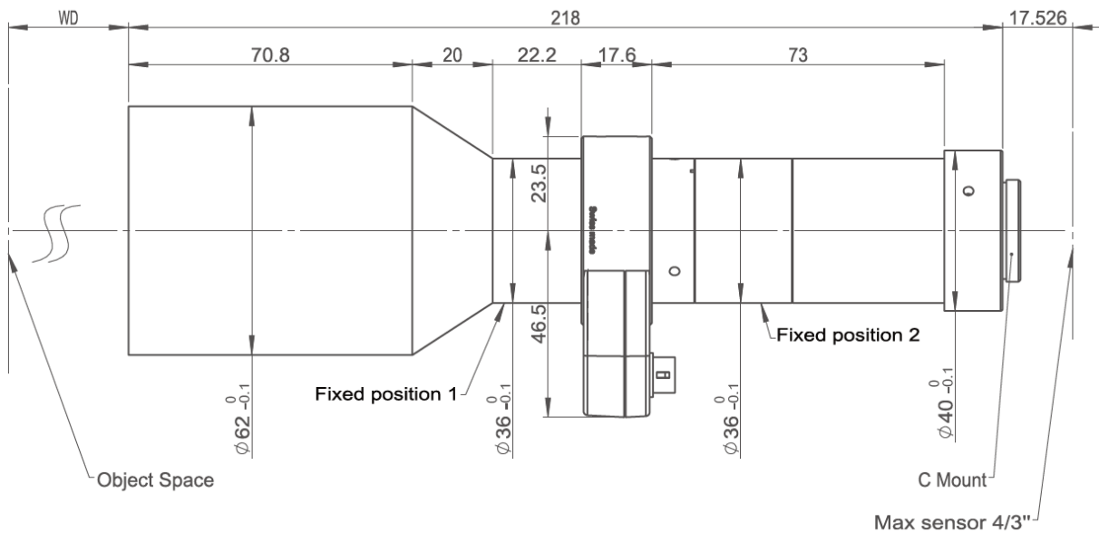
Figure 1: Mechanical drawing of the TS43-056-200-EL
