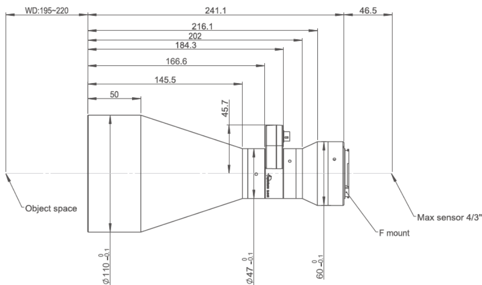
Figure 1: Mechanical drawing of the TS43F-0267-208-EL
