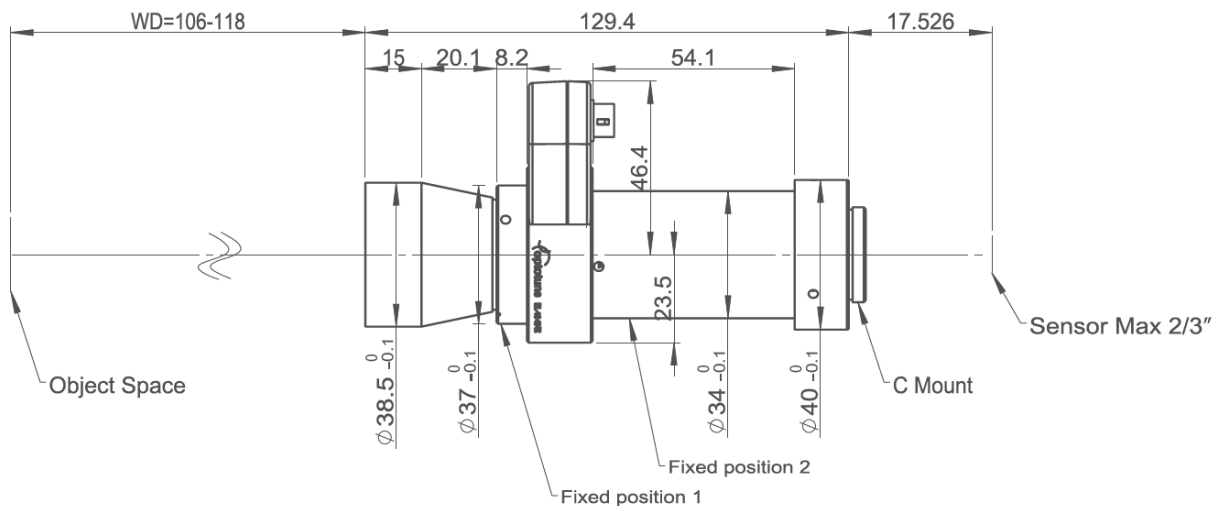
Figure 1: Mechanical drawing of the TST23-1.0-110-EL
