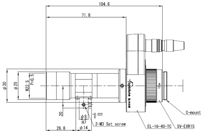
Figure 1: Mechanical drawing of the VS-TCH4-65-LQL1
