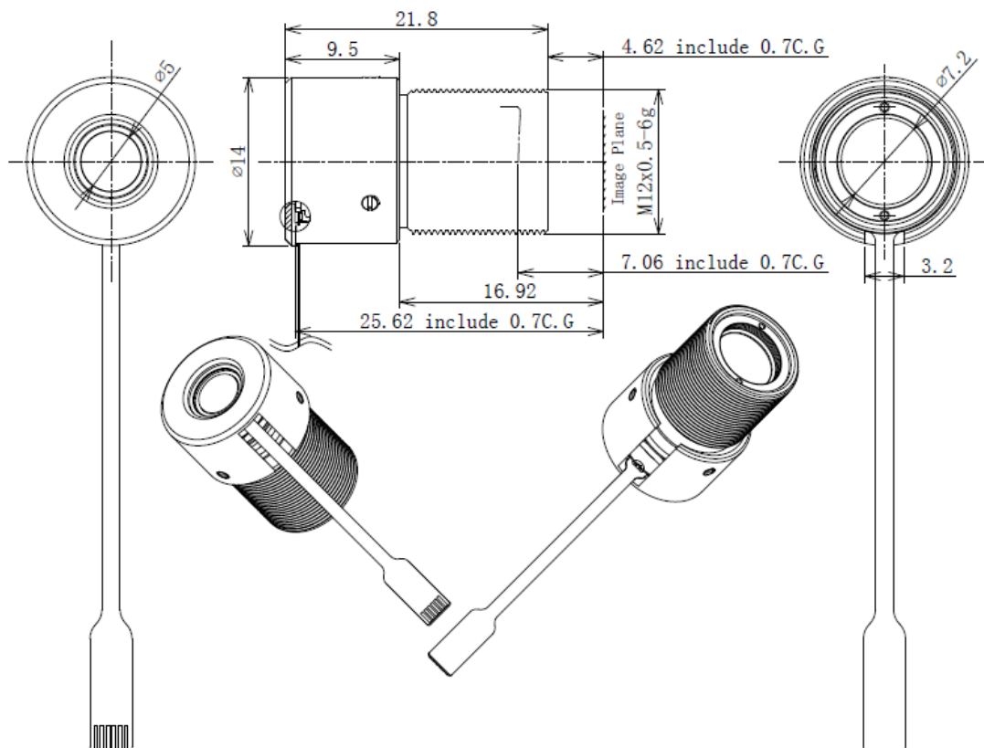
Figure 1: Mechanical drawing of the ELM-16-5.4-8-S
