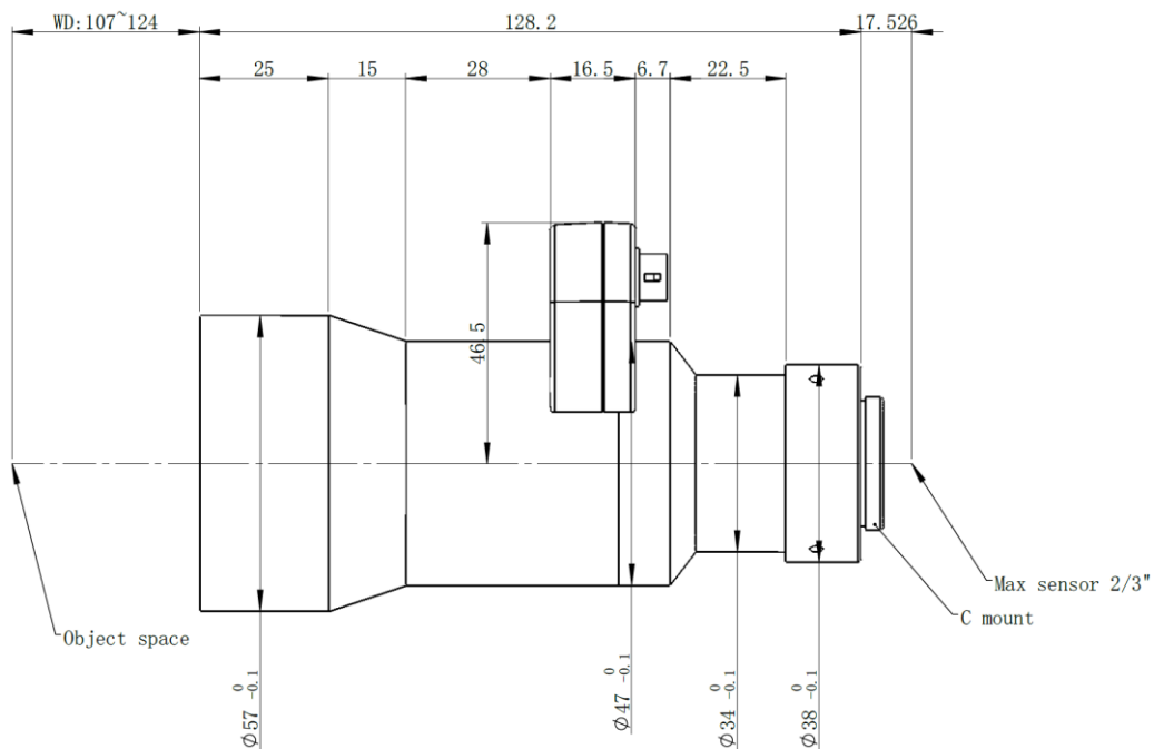
Figure 1: Mechanical drawing of the TST-S-23-036-115-EL
