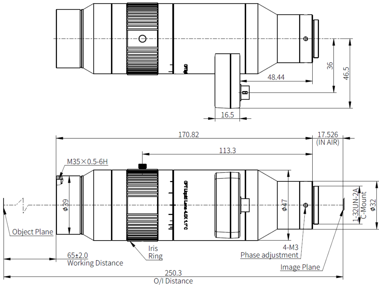
Figure 1: Mechanical drawing of the OPT-HP40-LQLTC-65
