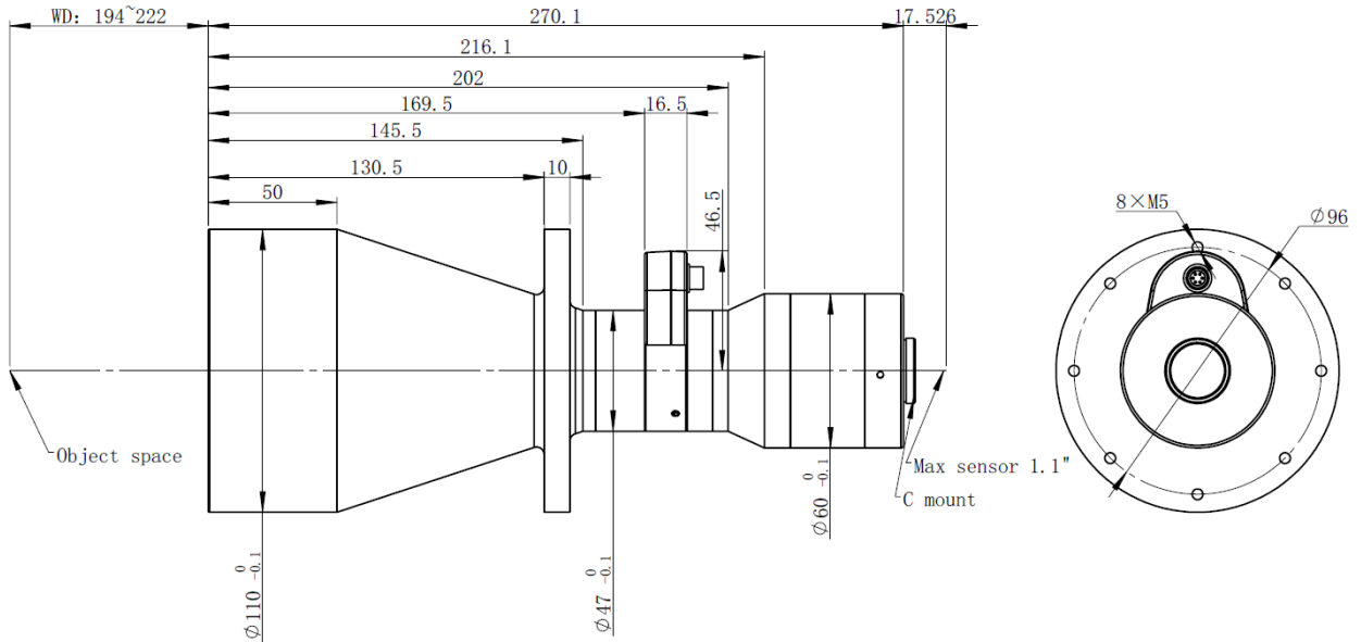
Figure 1: Mechanical drawing of the DTLP-11-0267-208 (unit: mm).
