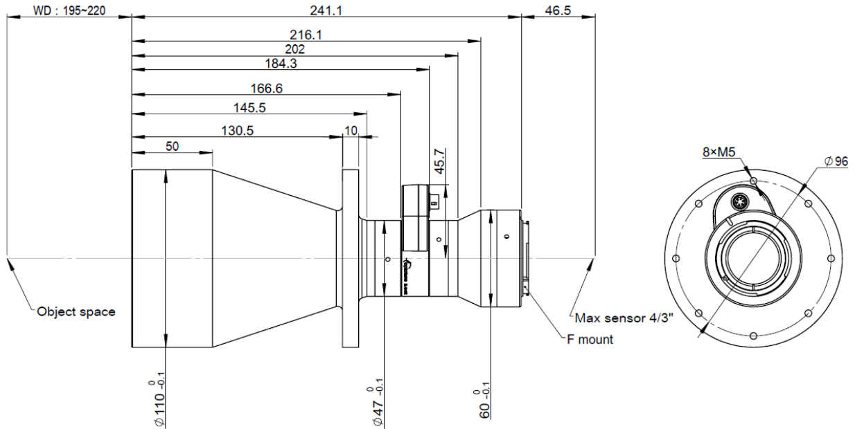
Figure 1: Mechanical drawing of the DTLP-43F-0267-208 (unit: mm).
