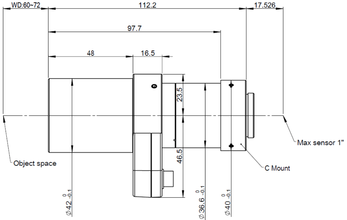
Figure 1: Mechanical drawing of the DTLP-S-1-0638-70 (unit: mm).
