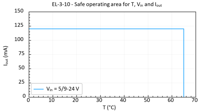
Figure 7: Guaranteed drive current for EL-3-10 lens available from ECC-1C.
