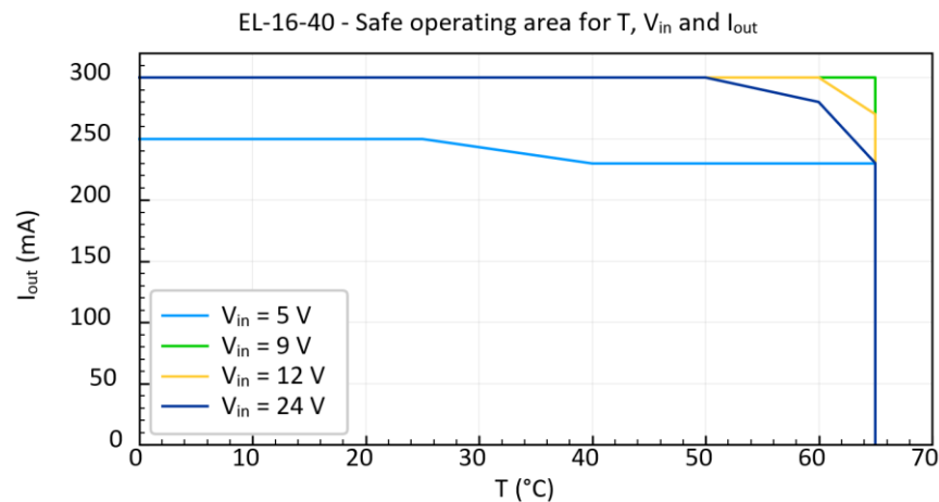
Figure 5: Guaranteed drive current for EL-16-40 lens available from ECC-1C.
