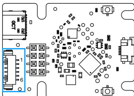
Figure 3: Pin out of PicoBlade 532610671
