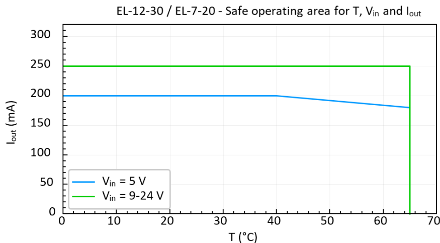
Figure 6: Guaranteed drive current for EL-12-30 / EL-7-20 lens available from ECC-1C.
