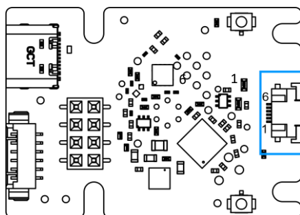
Figure 4: Electrical connections of flex cable connector.
