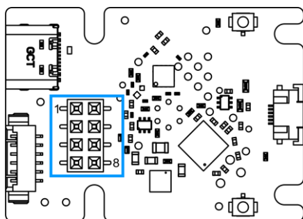
Figure 2: Pin out of M20-7810445R connector
