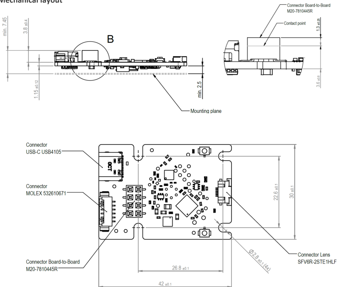
Figure 1: Mechanical drawing of ECC-1C OEM
